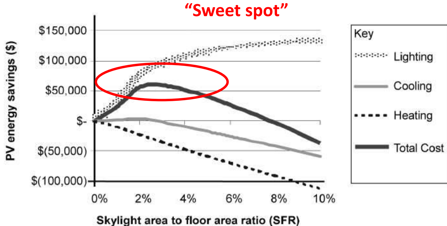
Figure 3-10 – Present Value Savings of Skylight 50,000 ft² Warehouse in Sacramento
